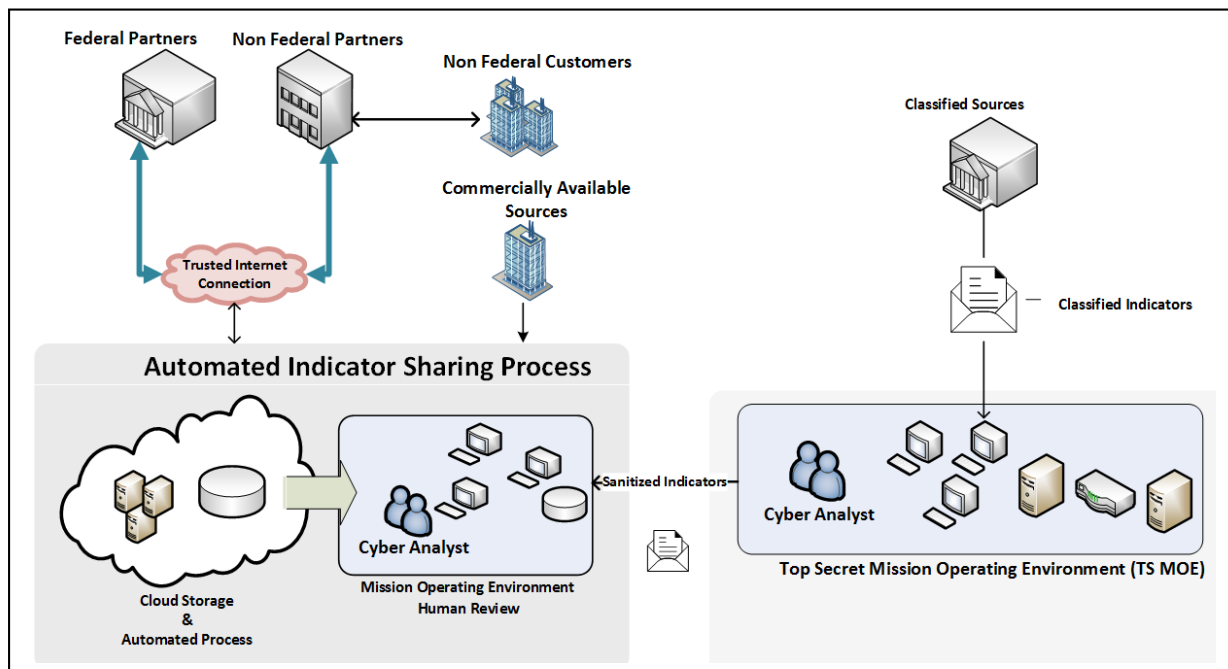
Figure 1: AIS and National Cybersecurity Protection System Cyber Threat Indicator Data Flow
